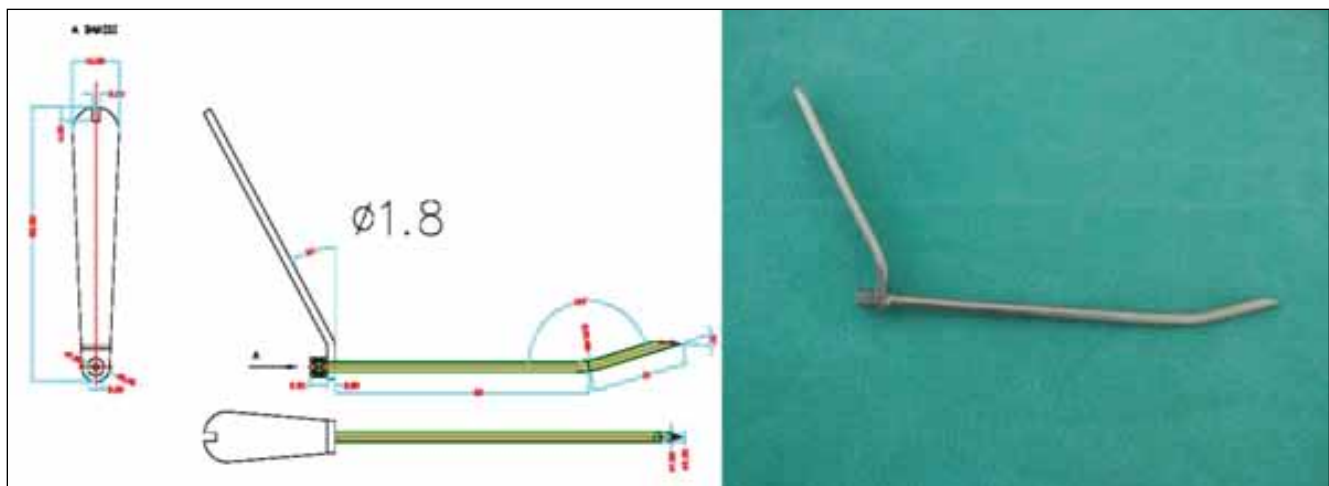
Figure 1: Guide tube that we used for anterior odontoid screw fixation.
